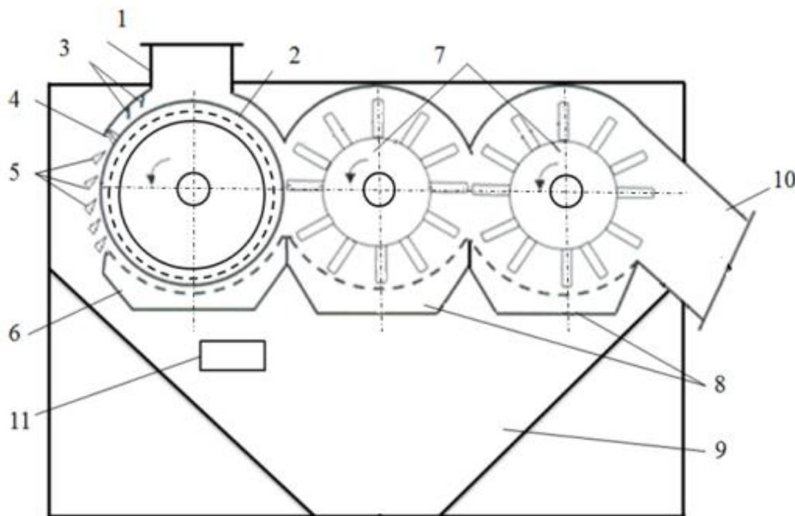
1- rasm. MT-02 rusumli kombinatsiyalangan turdagi momiq tozalagichning sxemasi
